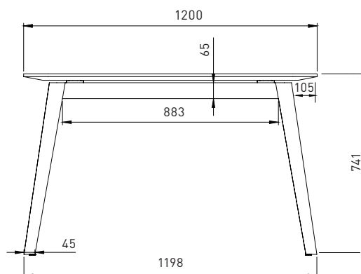
Sloping edges
