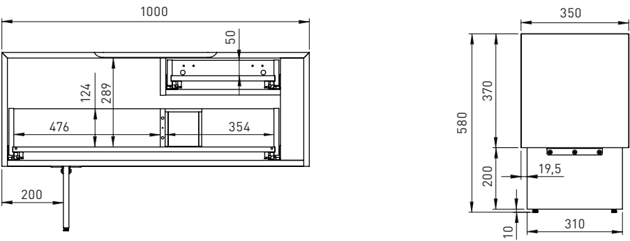
Desk pedestal
